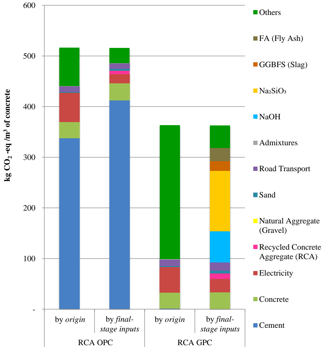
Figure 8: Decomposition of LCIs by origin and by final-stage inputs for ordinary Portland cement (OPC) concrete and geopolymer concrete (GPC)
