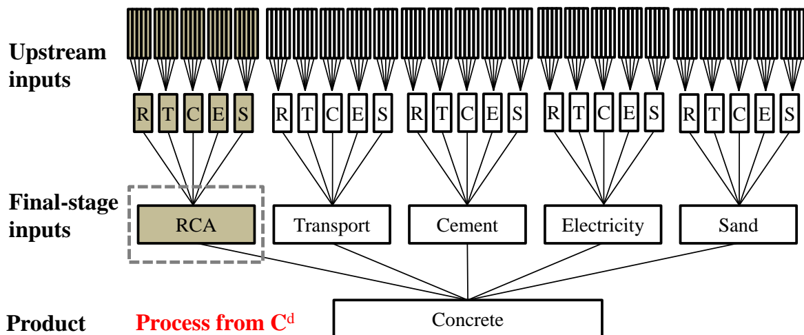
Figure 10: Recycled concrete aggregate (RCA) contribution in the decomposition of LCIs by final-stage inputs method in the OPC concrete production
