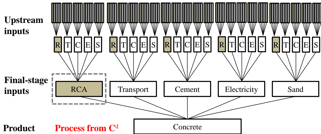
Figure 9: Recycled concrete aggregate (RCA) contribution in the decomposition of LCIs by origin method in the OPC concrete production
