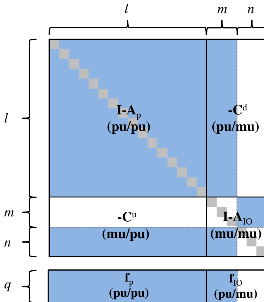
Figure 3: Integrated coefficient matrix (I-A_{IH}) of integrated hybrid LCA (blue shaded areas include non-zero values but may be sparsely populated; non-shaded areas contain zeroes; grey shaded areas represent 1's on the diagonal; pu= physical units; mu= monetary units)
